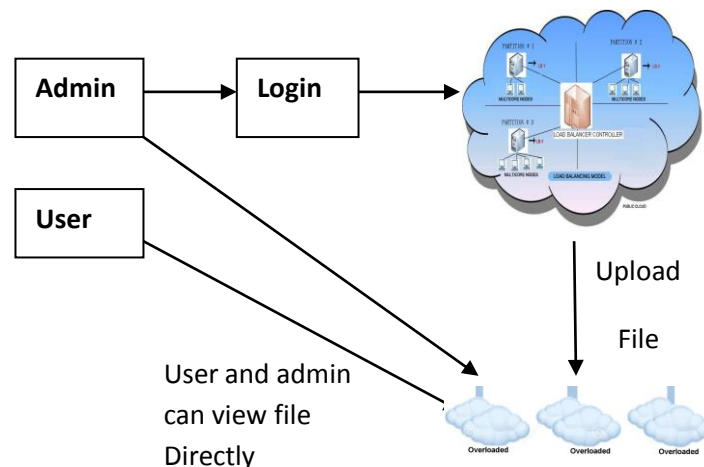
Fig1. Architecture of load balancing model based on cloud computing for heterogeneous partition
